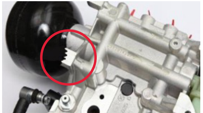
Holder broken handling damage
